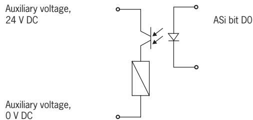
Figure 5: Connection example guard locking control via ASi bit D0 (guard locking for process protection only)
